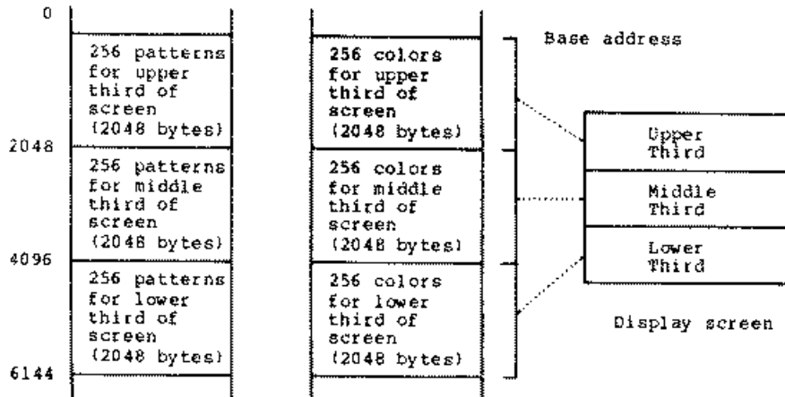
Pattern generator table
