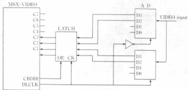
Digitize Block Diagram (GRAPHIC 5 mode)
