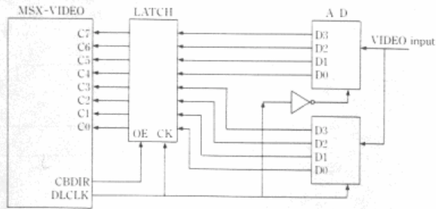
Digitize Block Diagram (GRAPHIC 6 mode)
